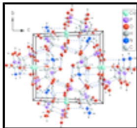
Fig. 2. Crystal packing of the title compound viewed down the a axis, showing the three-dimensional chain structure. Hydrogen bonds are shown as dashed lines.
